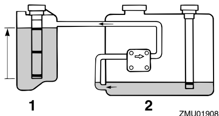
1. Motorns oljetank 2. Extern oljetank
