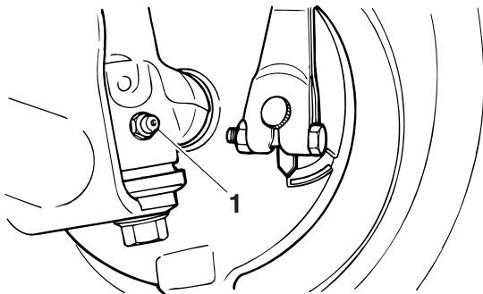
1. Grease nipple
