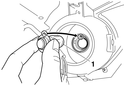
1. Headlight bulb
