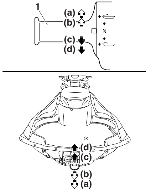
1 Q.S.T.S. selector
